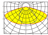
BELFRY PRO LIGHT DISTRIBUTION DIAGRAM
