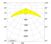
OVAL VERSION Light distribution elongated in one dimension, short in the other. Suitable for corridors.
