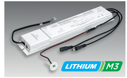
STANDARD OR SELF-TEST EMERGENCY CONVERSION PACK WITH LITHIUM (LiFePO4) BATTERY - SEE PAGE 69
