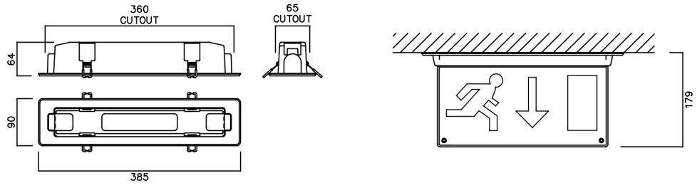
RECESSED MOUNTING KIT (NAL/RMK)
